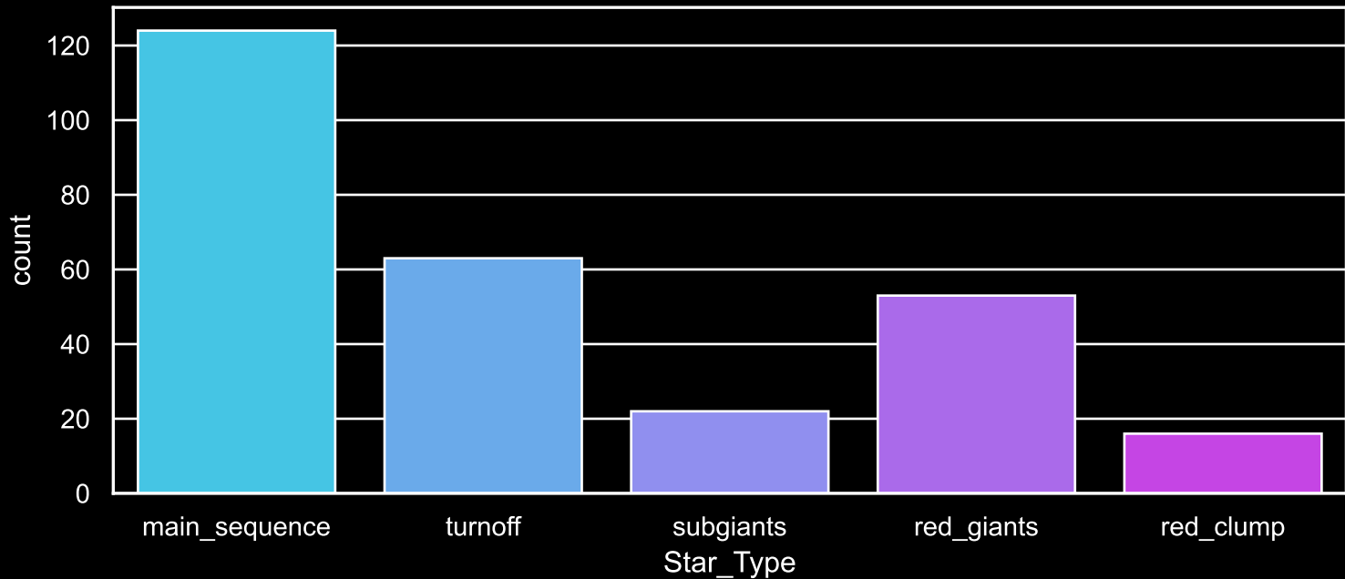
Field [85] Count plot of Star Type
