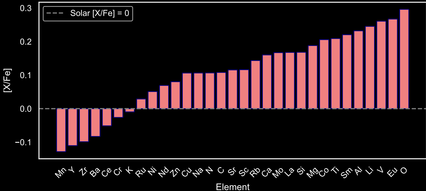
Abundance Pattern for GALAH Red Giants: Star Field [85] (N=69)
