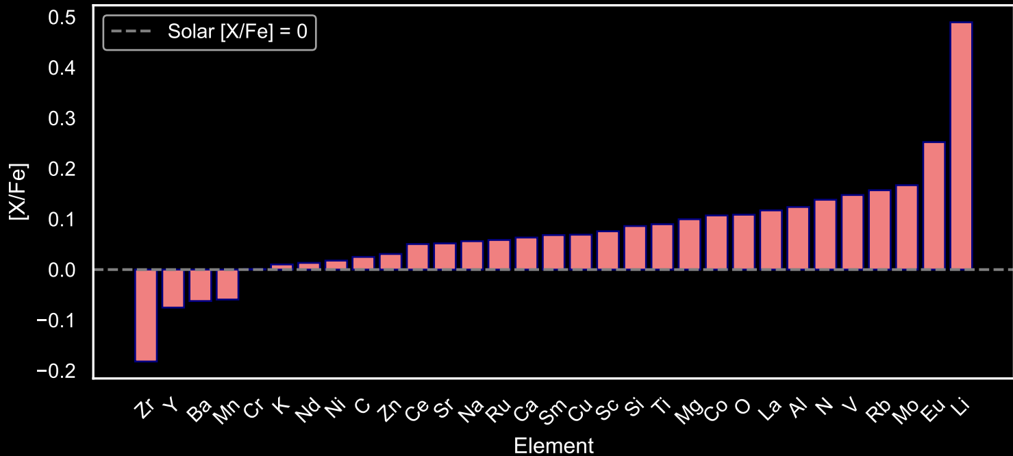
Abundance Pattern for GALAH Star Field [85] (N=278)
