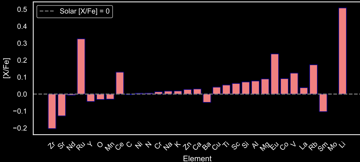
Abundance Pattern for GALAH Main Sequence Stars: Star Field [85] (N=124)
