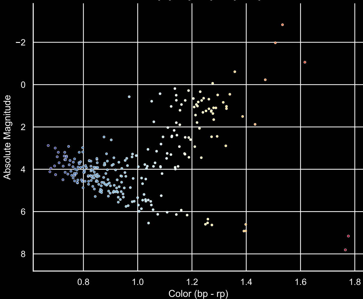
GALAH Hertzprung-Russel Diagram Field [85] Ra [320.0] Dec [-26.21]
