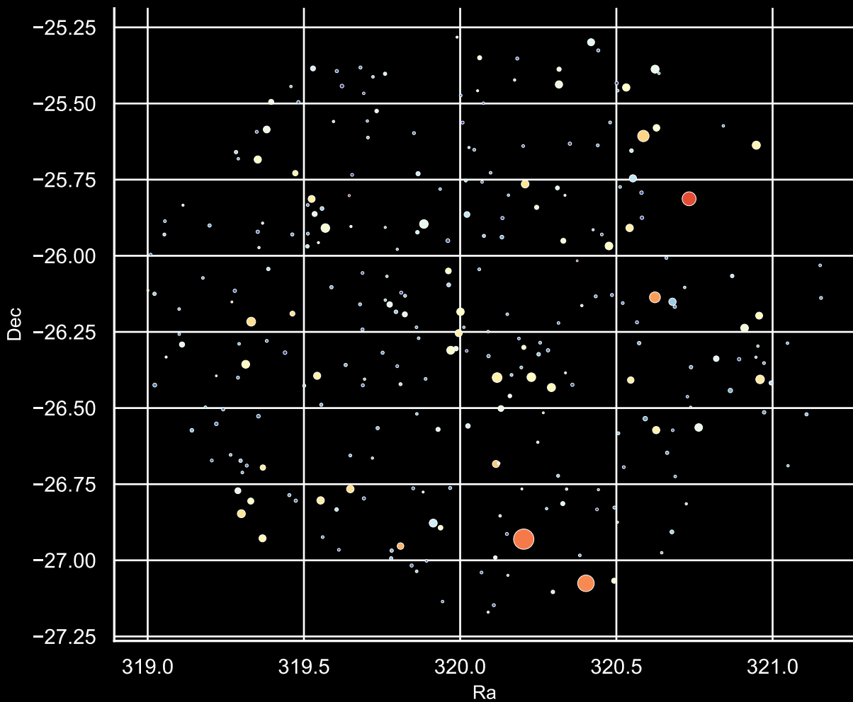
Field [85] Ra [320.0] Dec [-26.21] Stars: 278
